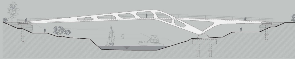
SOUTH ELEVATION 1:250
